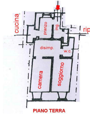
PIANO TERRA
