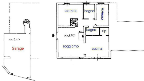
PIANO SEMINTERRATO
