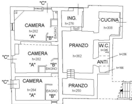
PIANO TERRENO
